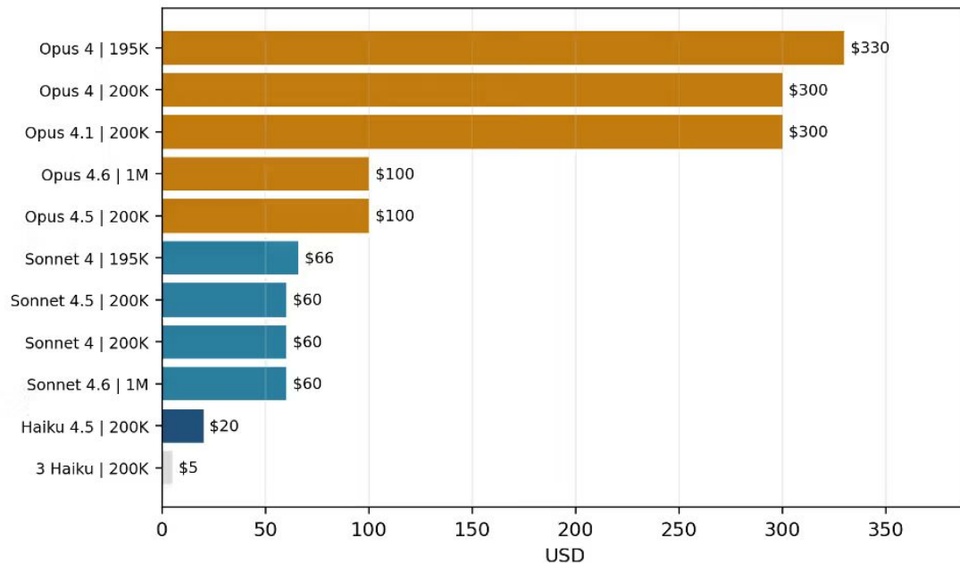
Illustrative Daily Cost by Latest Observed Model Variant (10M input + 2M output tokens)
